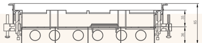
Cut out dimension 313x128mm
