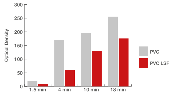
Smoke Release (ISO5659-2:2012) - Standard PVC vs PVC/LSF*
